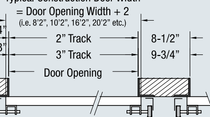
Reverse Angle Track Steel / Masonry Jambs
